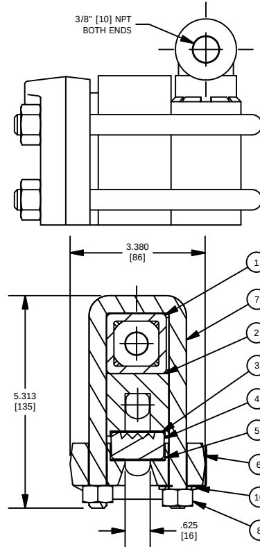
SECTION X-X SERIES RH-20
